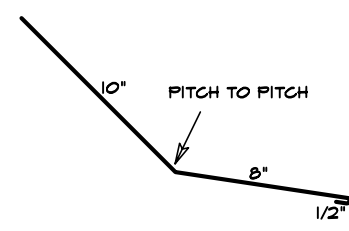
20b TRANSITION LOW HIGH
