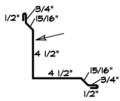
15 OUTSIDE CORNER
