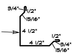
16 BASE TRIM
